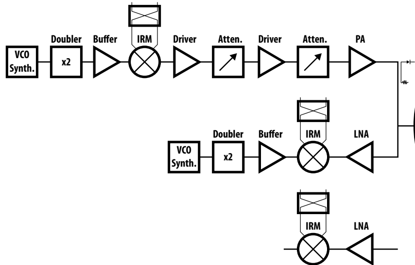
Microwave Link Packaged Suggested Solution 10-11 GHz
