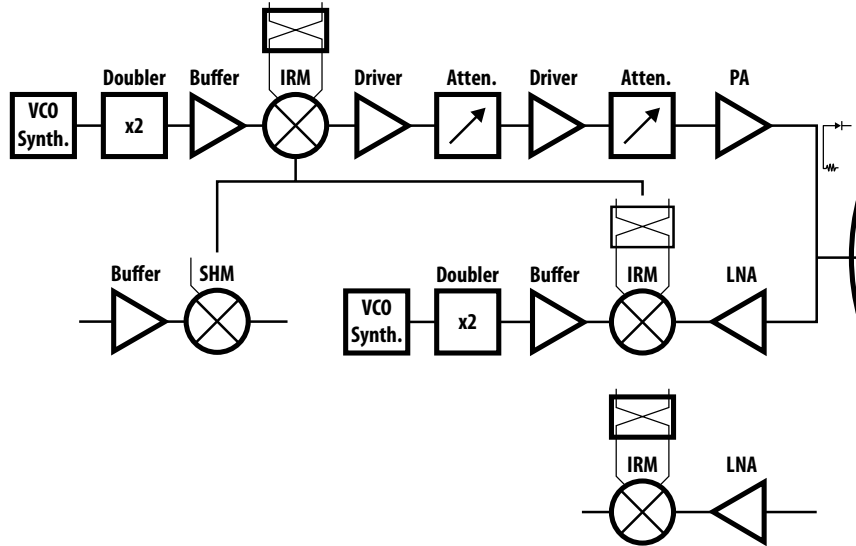
Microwave Link Packaged Suggested Solution 23 GHz
