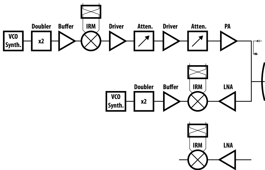
Microwave Link Packaged Suggested Solution 28 GHz
